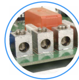
Terminals 16 mm 2
