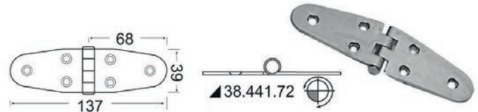
Scharnier type 9
