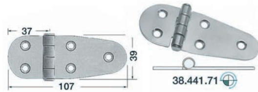
Scharnier type 8
