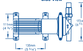
Plan View
